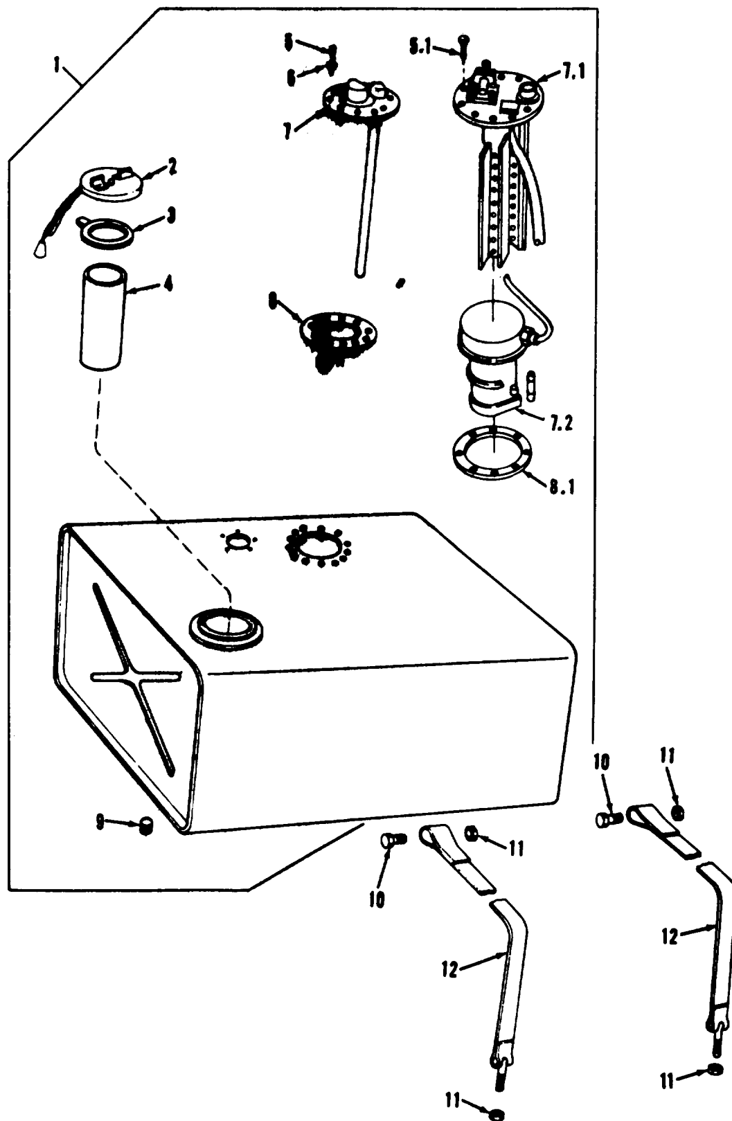
Figure 8. Fuel tank assembly.
