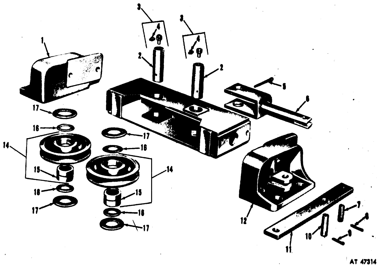
Figure 219. Rear winch tensioner assembly.
