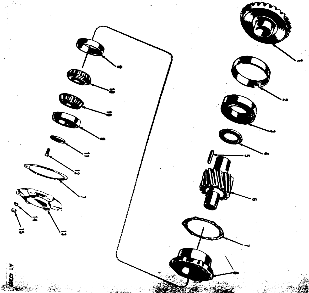
Figure 70. Differential helical drive pinion and bearings.
