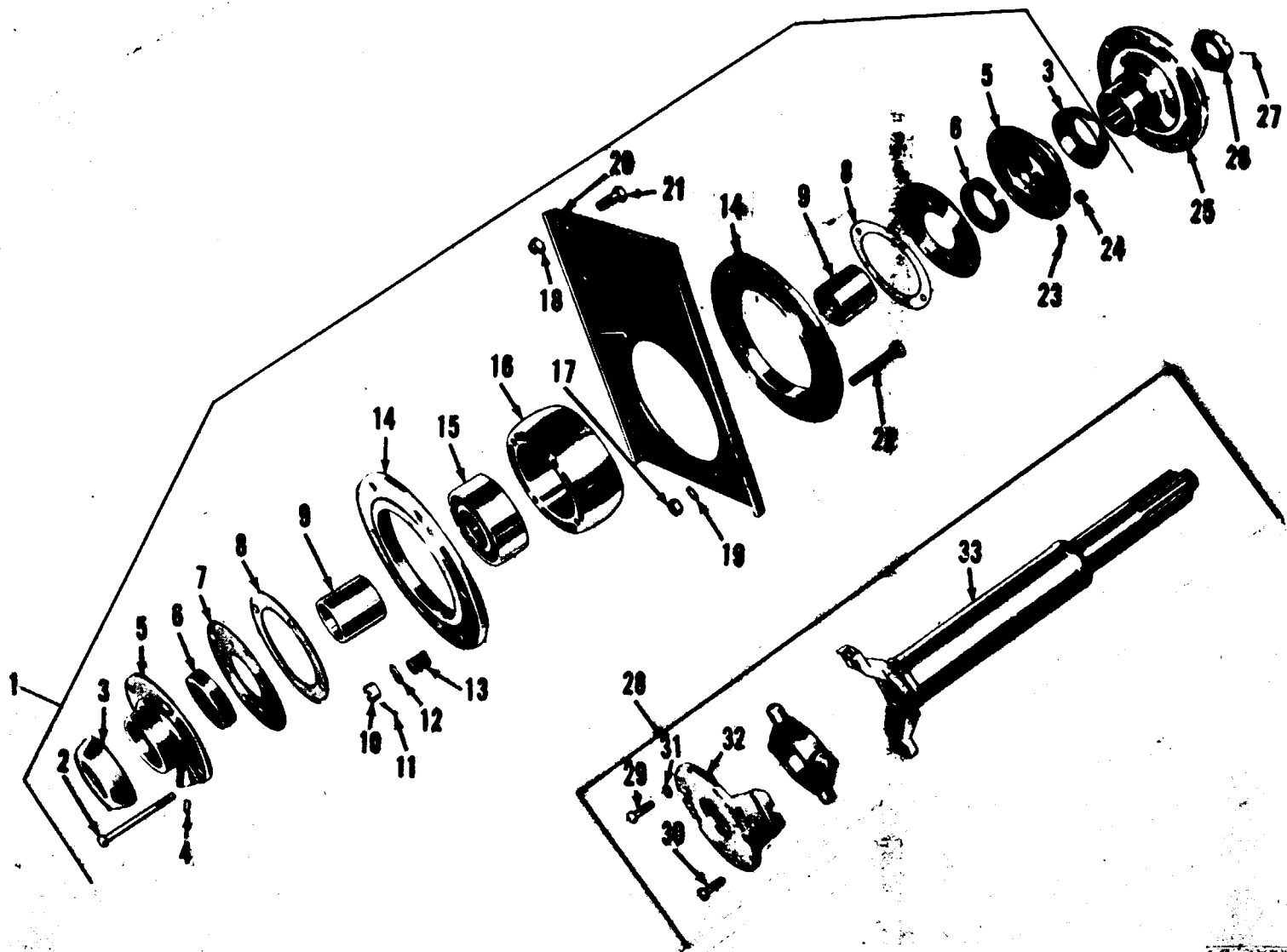
Figure 61. Propeller shaft—transfer to center bearing assembly.
