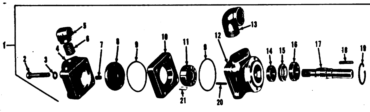
Figure 236. Boom hoist hydraulic oil motor.
