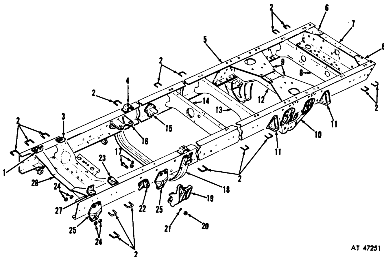
Figure 109. Frame assembly.
