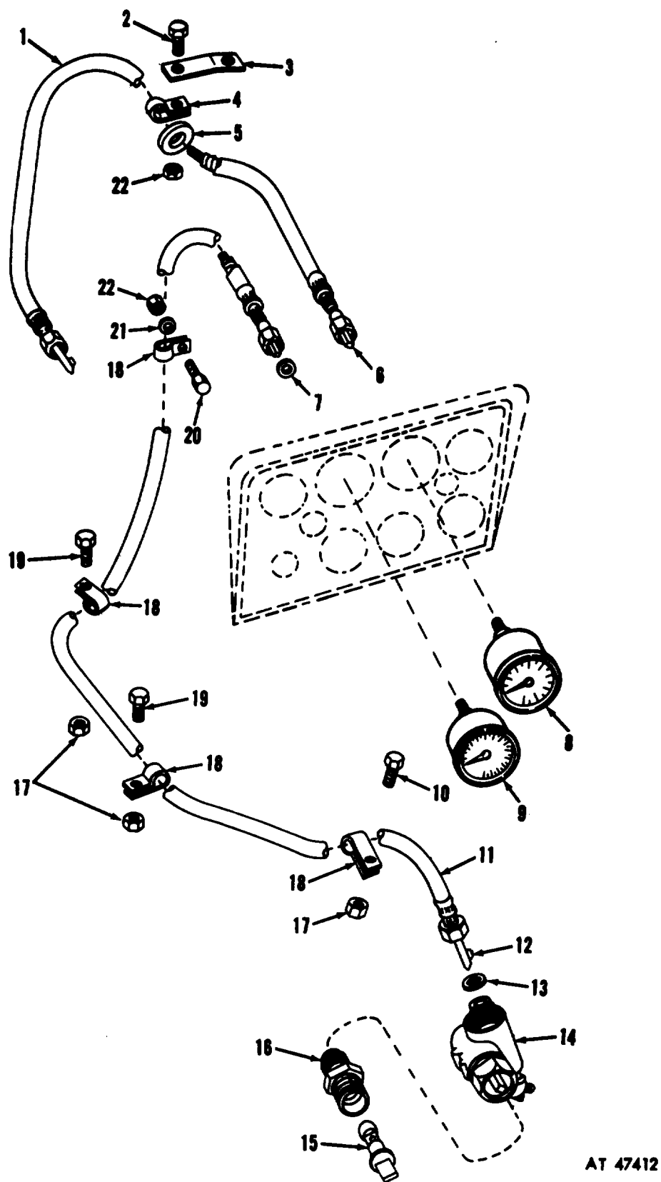
Figure 309. Speedometer and tachometer shafts and related parts.
