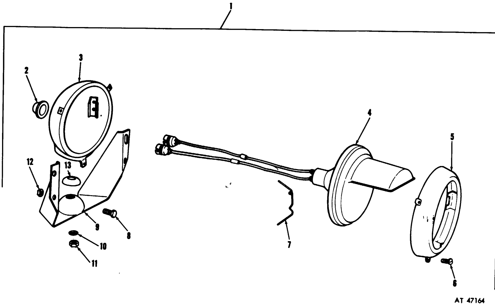
Figure 23. Blackout headlight assembly.
