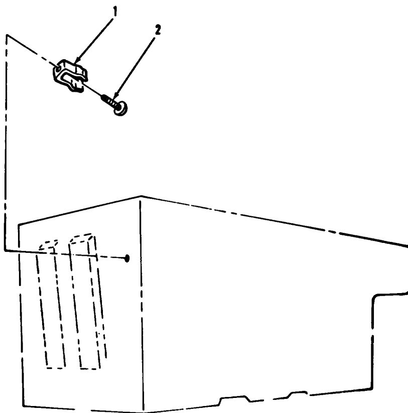
Figure 187. Van body end panel and stowage retainer.
