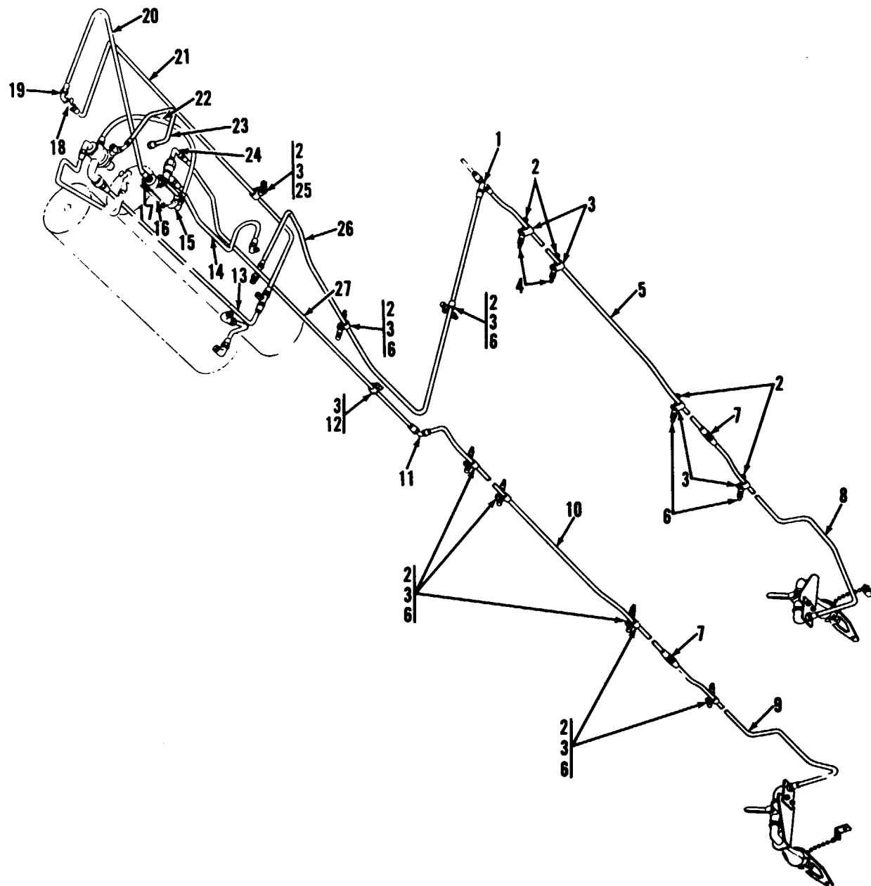
Figure 86. Air lines (rear).
