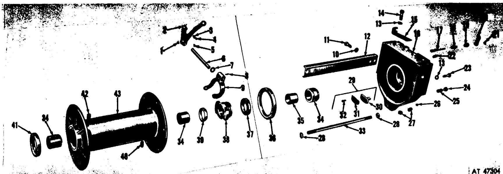
Figure 209. Front winch drum and end frame.
