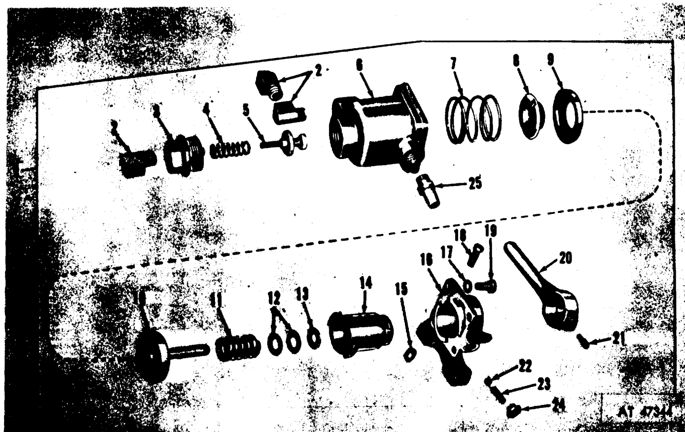
Figure 253. Brake valve.
