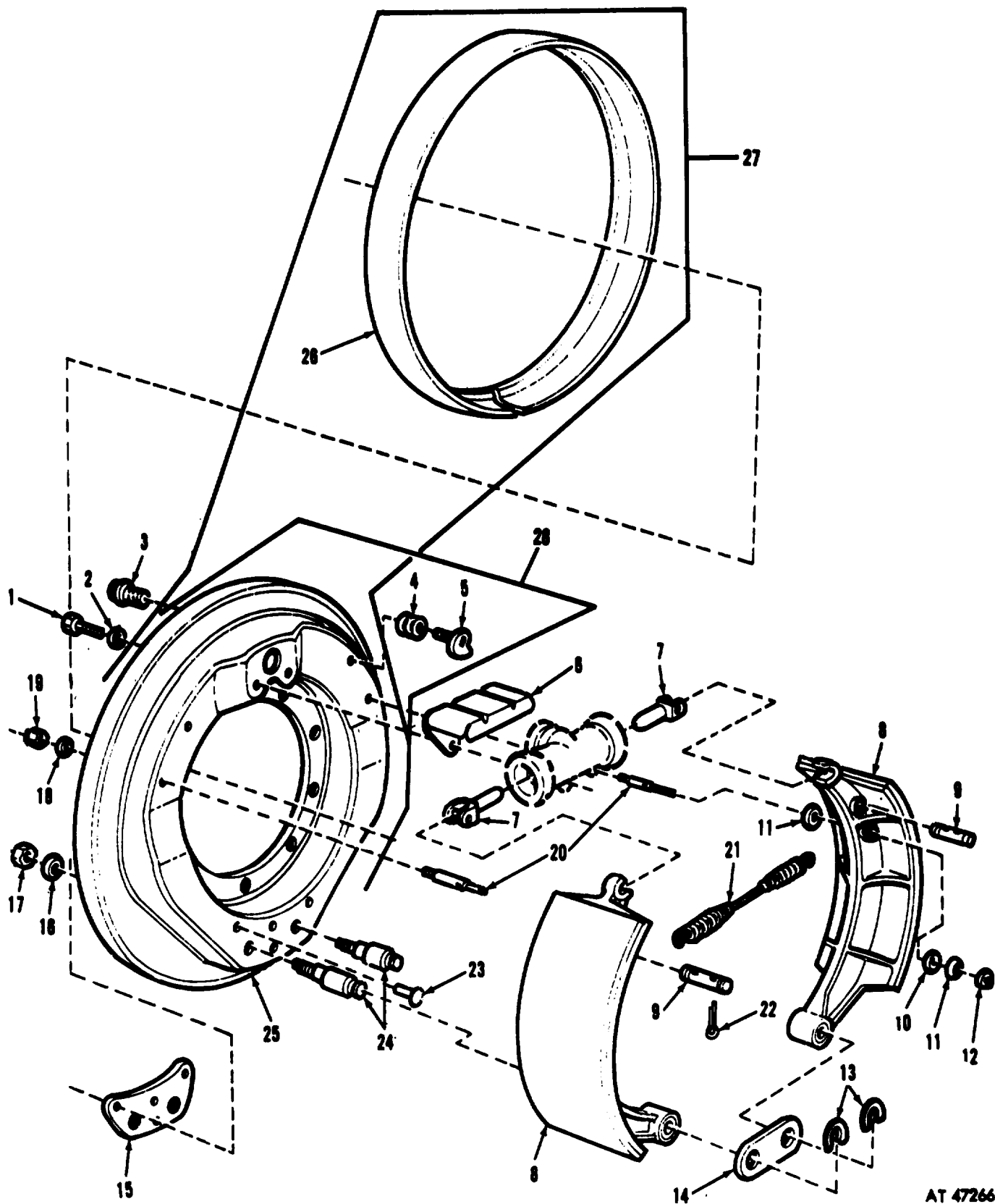
Figure 79. Service brakes.
