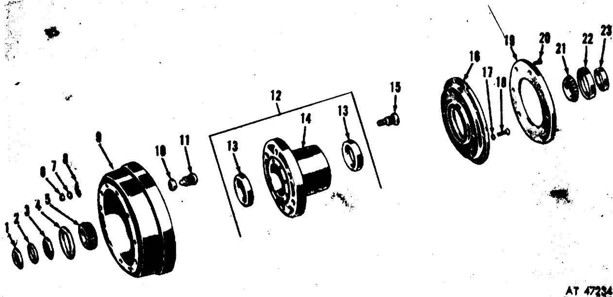
Figure 95. Rear axle hub assy, drum and related parts.
