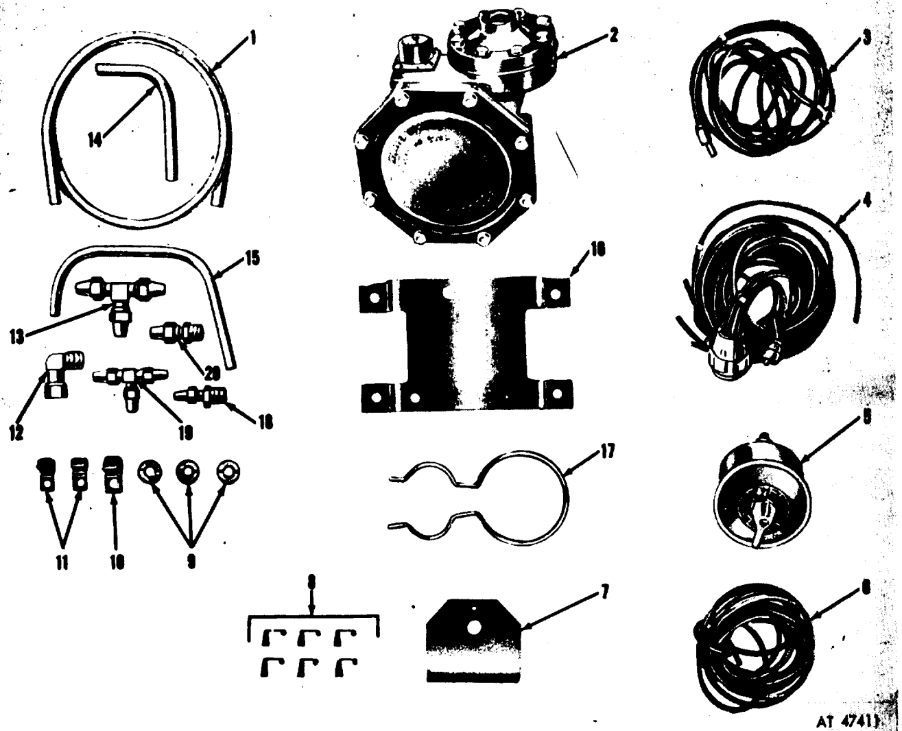
Figure 308. Electric brake components.
