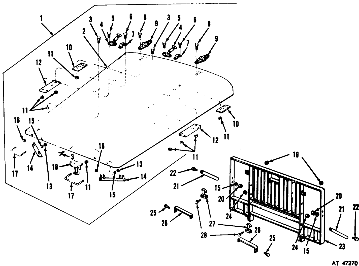
Figure 129. Hood assembly and related parts.
