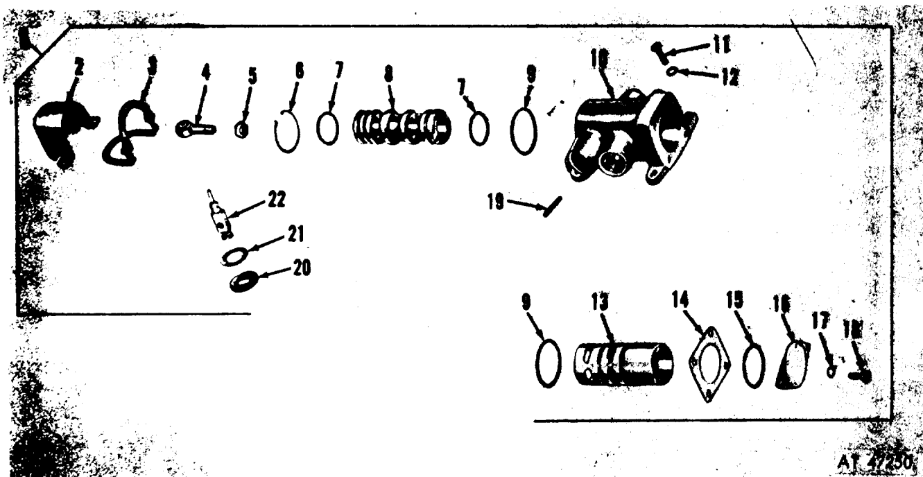
Figure 108. Steering gear hydraulic control valve assembly (component of figure 102).
