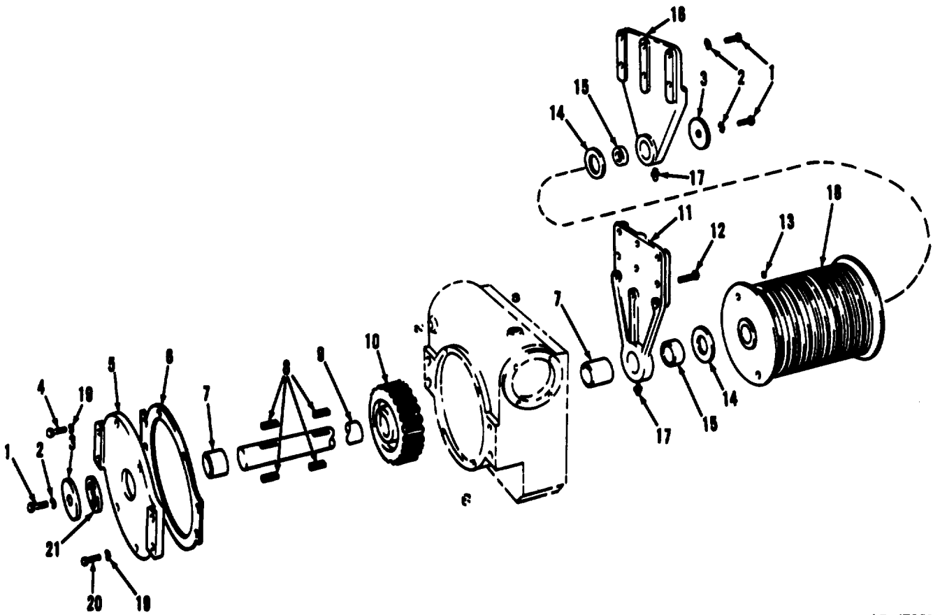
Figure 260. Hoist winch.
