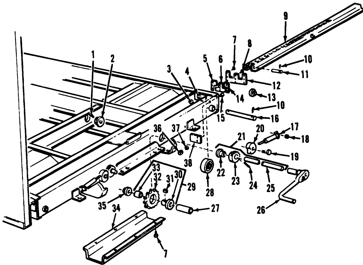
Figure 174. Underframe and related parts.
