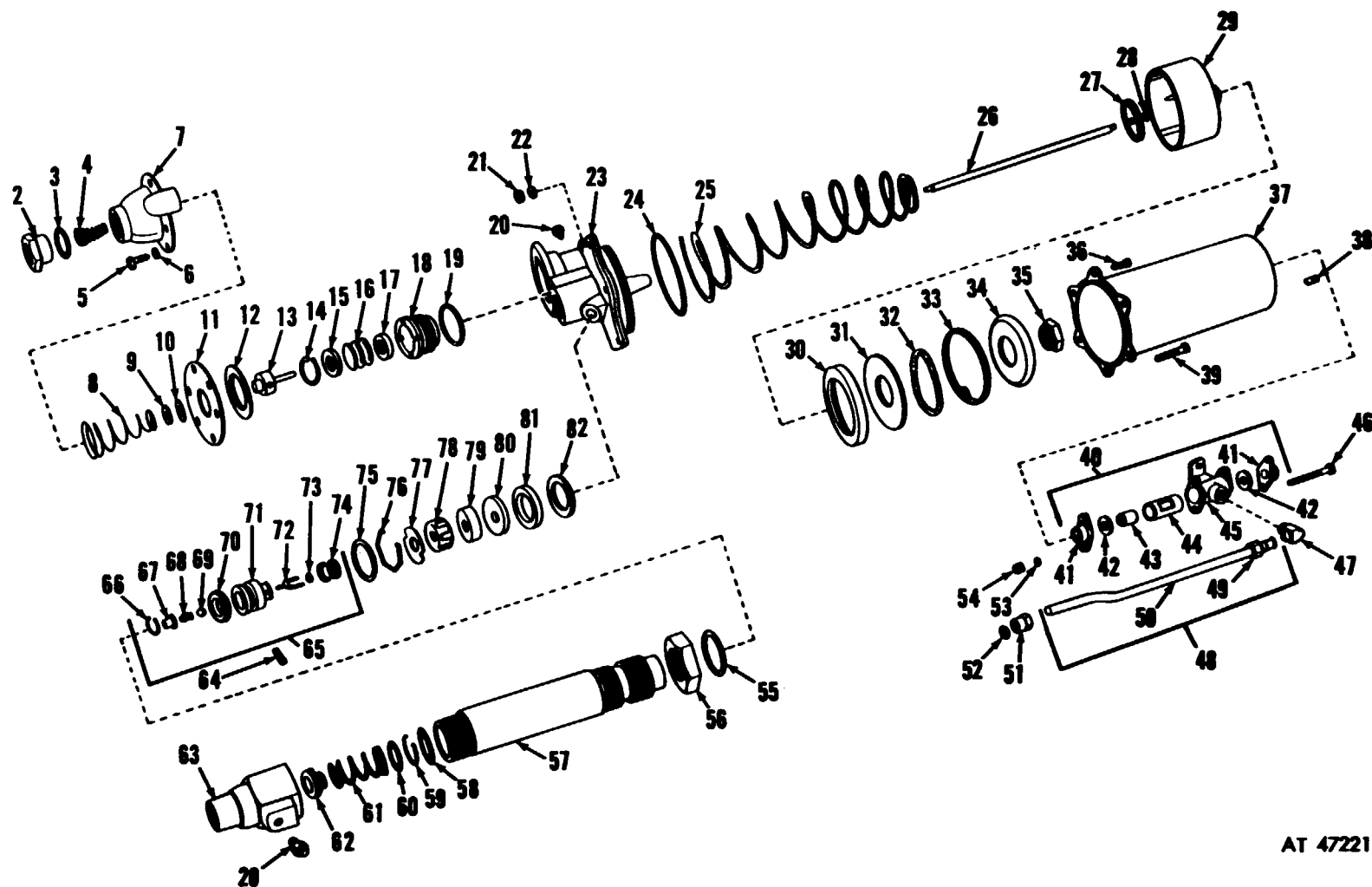
Figure 82. Hydraulic air cylinder.
