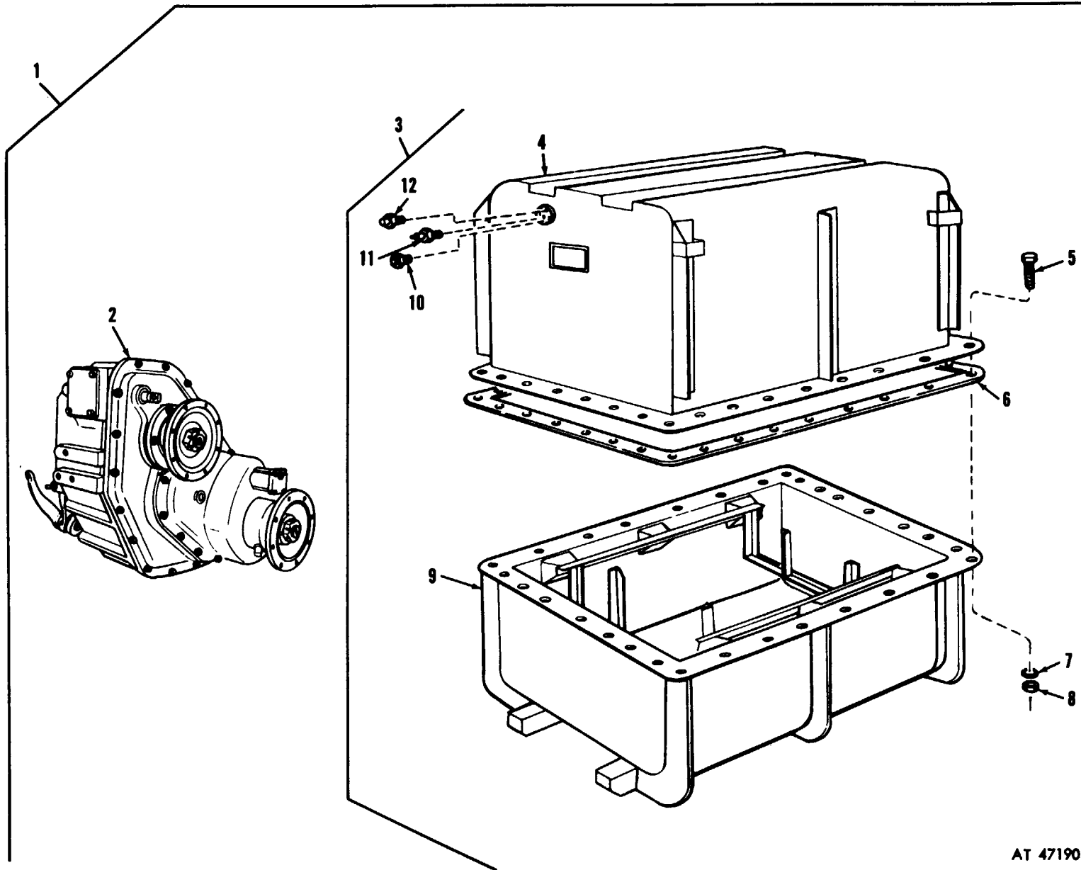
Figure 50. Transfer and container assembly.
