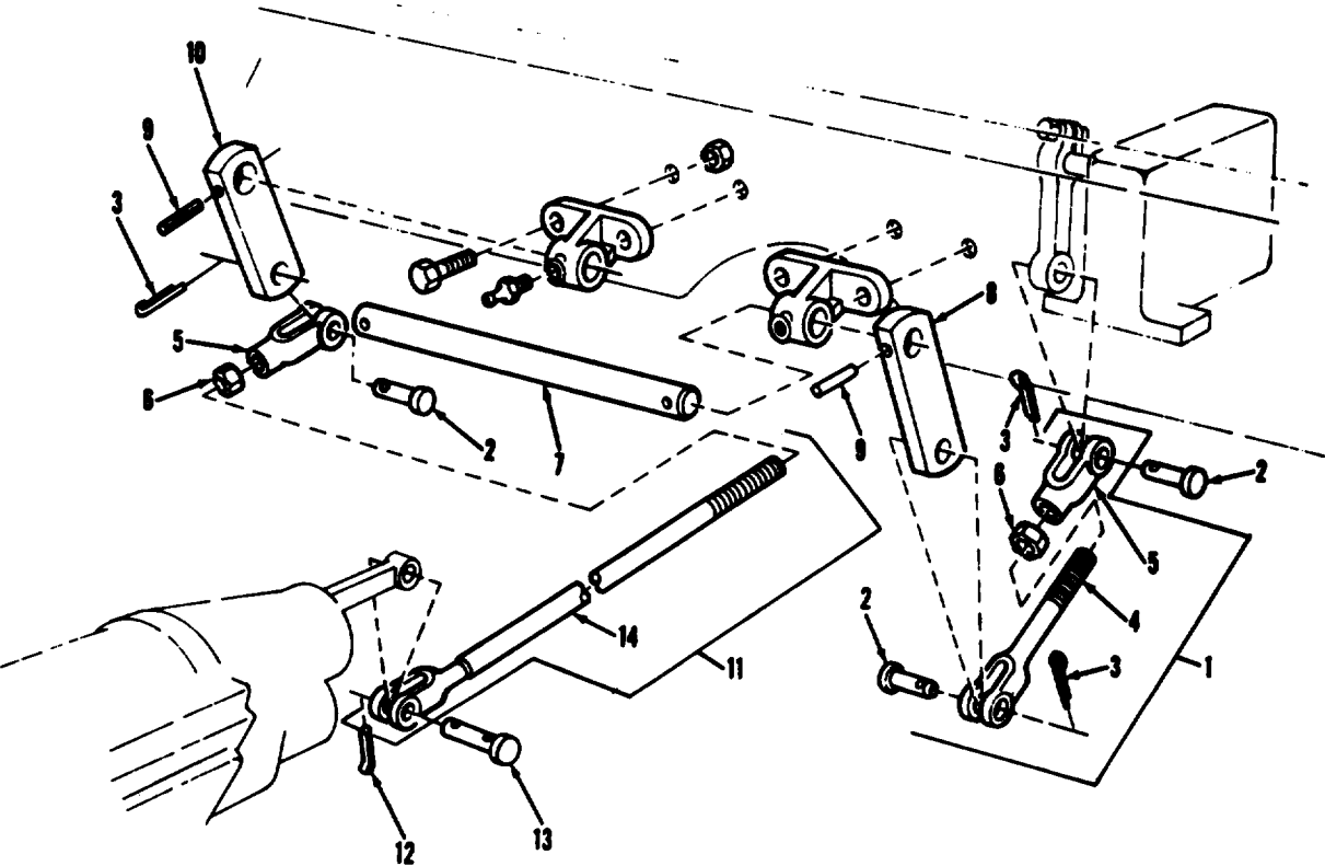
Figure 234. Dump control box rod and power takeoff control and shafts.
