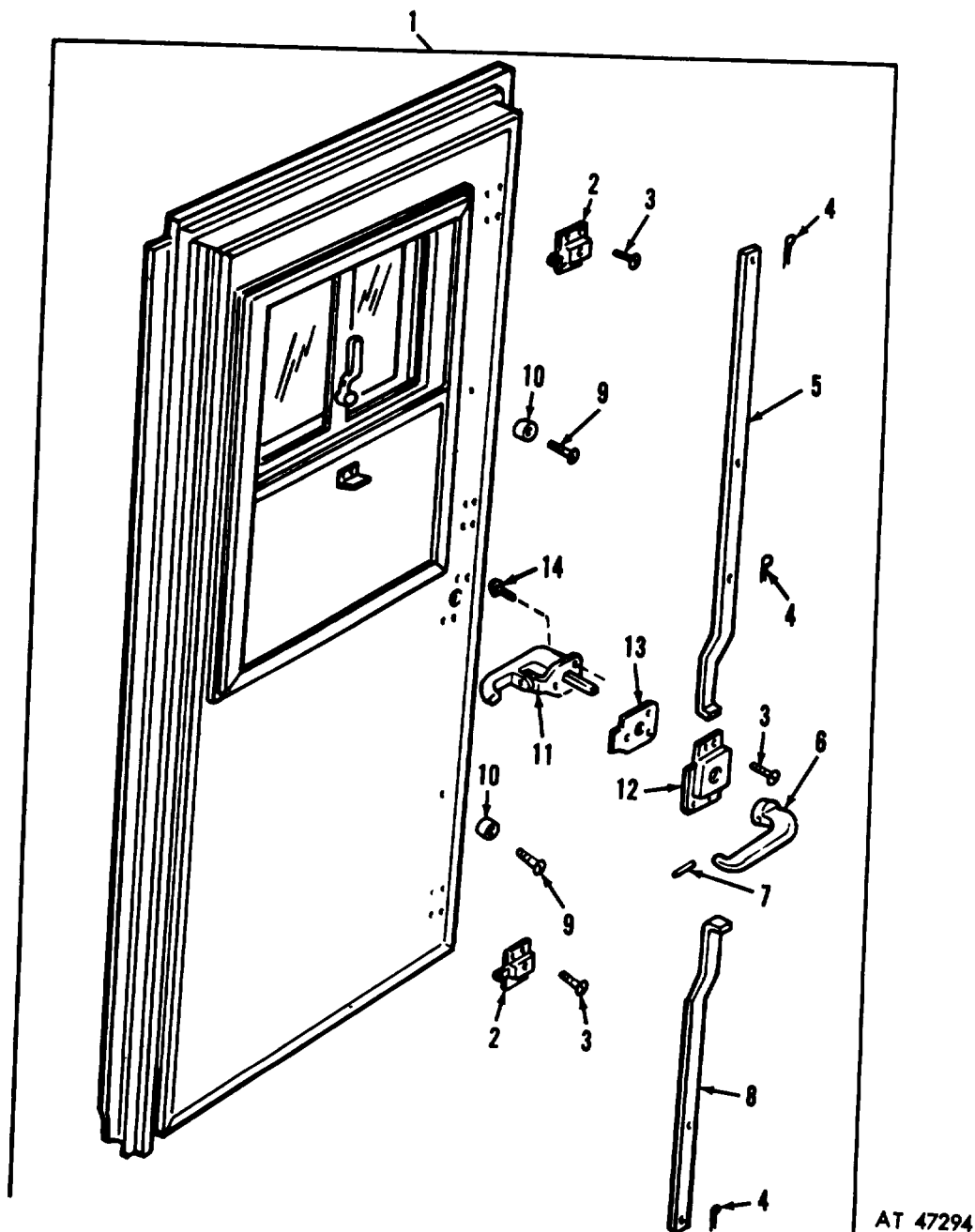
Figure 168. Side door assembly.
