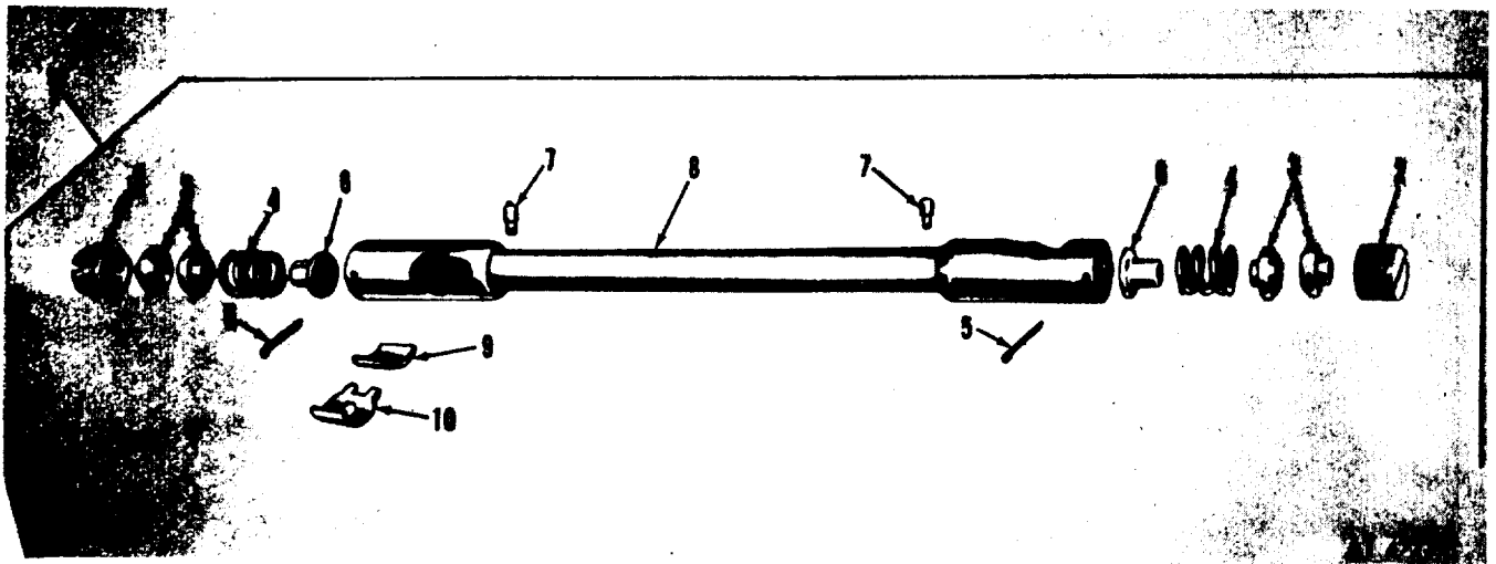
Figure 100. Drag link assembly.
