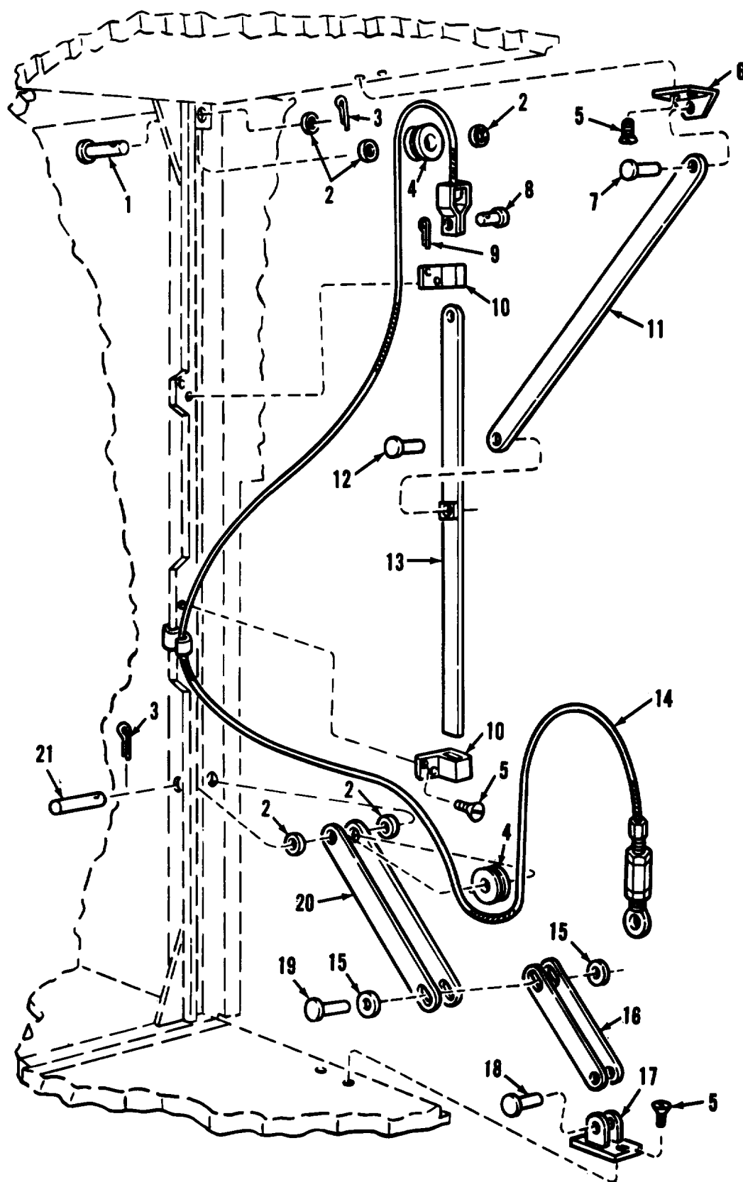
Figure 170. Counter balance assembly.
