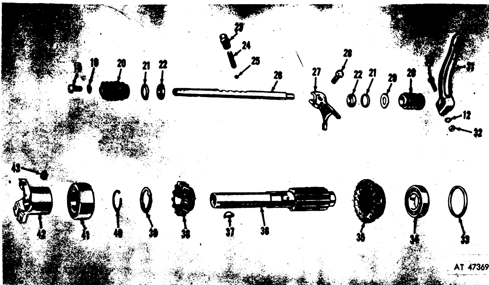
Figure 274. Transmission power takeoff assembly (2 of 3).
