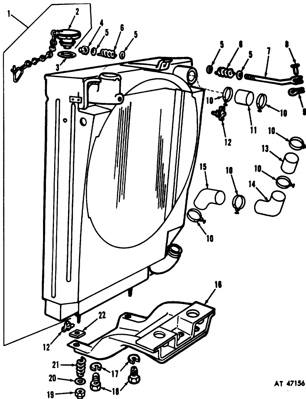
Figure 15. Radiator (gasoline).
