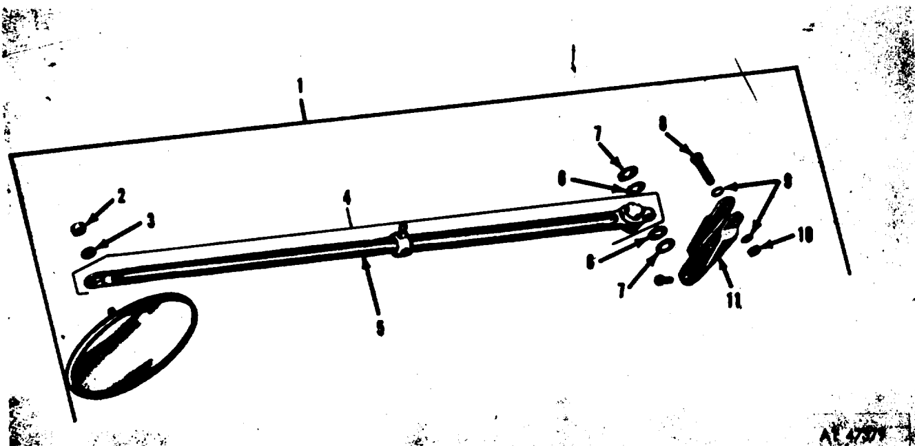
Figure 283. Right and left mirror assembly.
