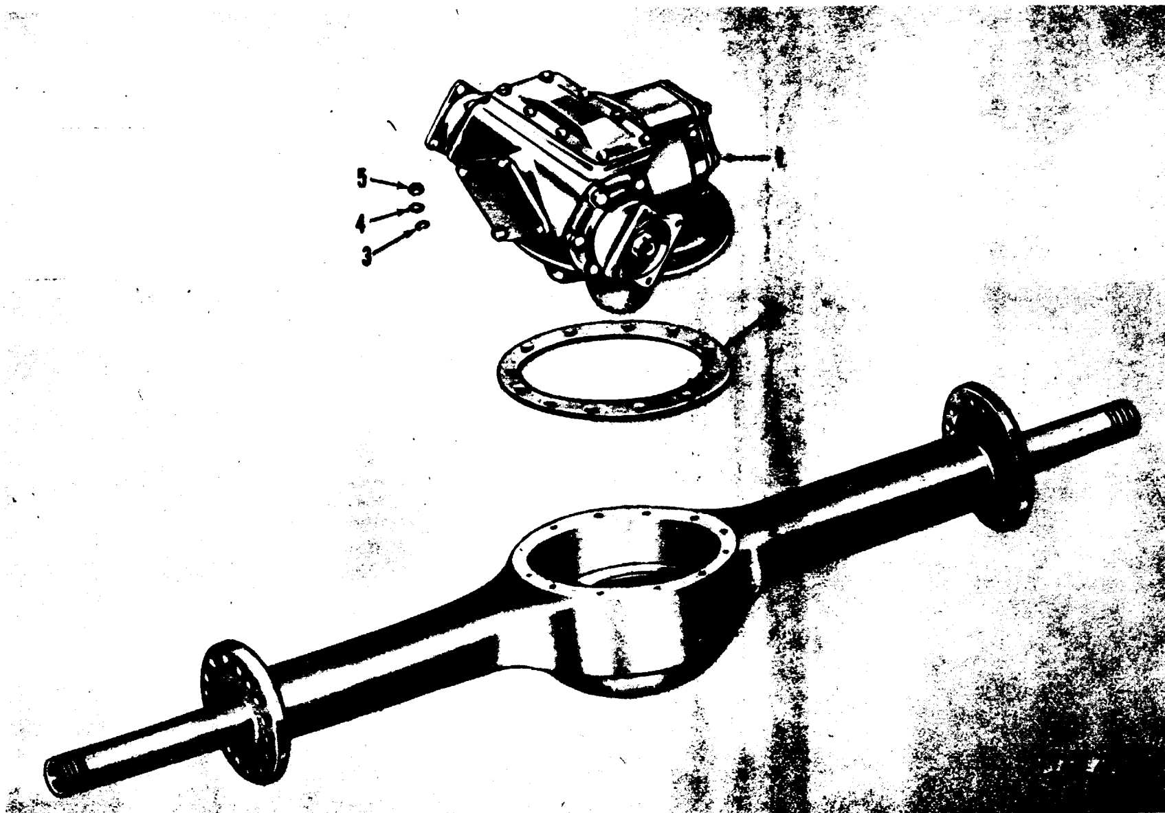
Figure 66. Differential carrier assembly.
