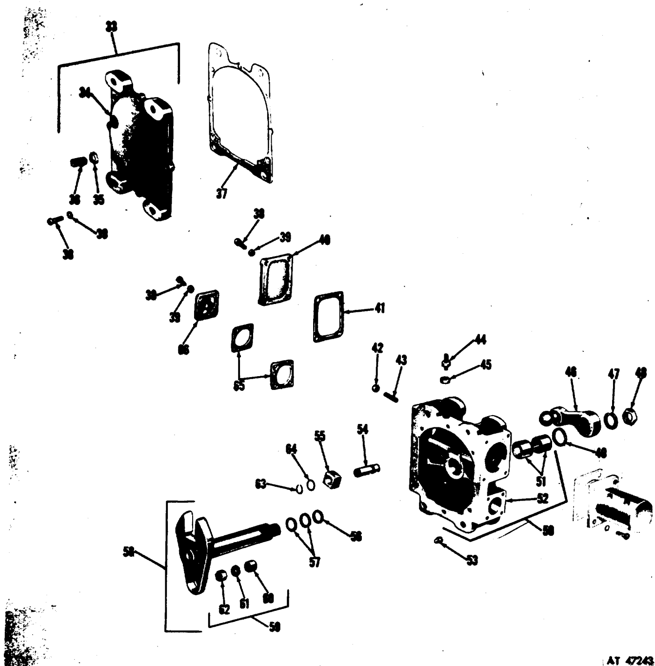
Figure 102. Steering gear assembly (3 of 3).
