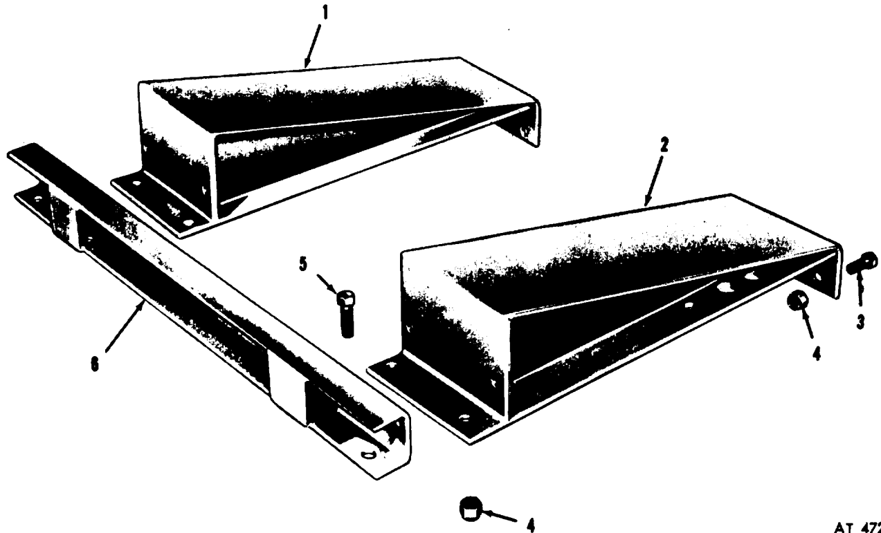
Figure 121. Fifth wheel approach plates.
