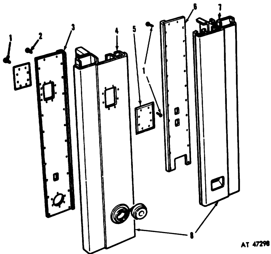
Figure 172. Rear wall assembly.
