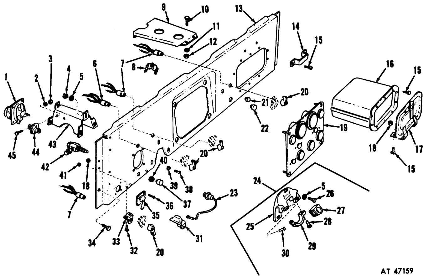
Figure 18. Instrument panel.
