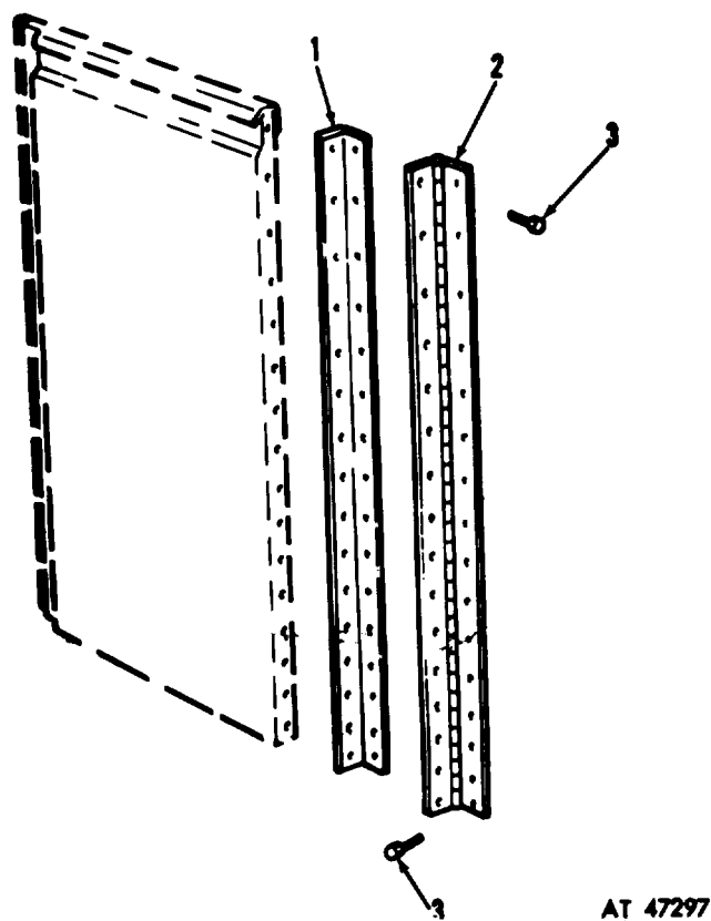
Figure 171. Door assembly end panel.
