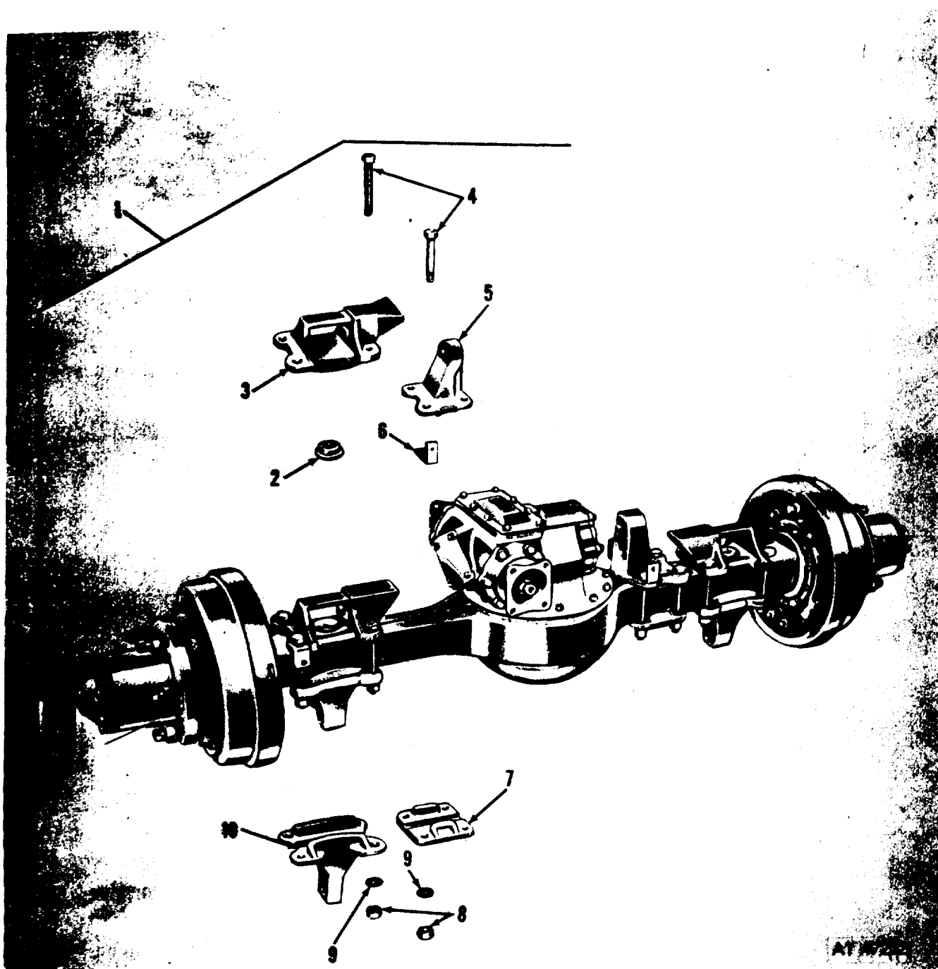
Figure 73. Rear axle assembly.
