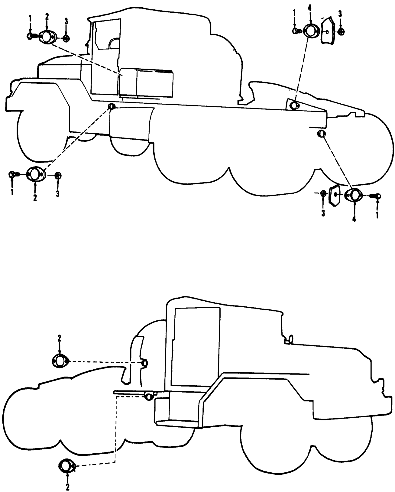
Figure 291. Tractor reflector assembly.
