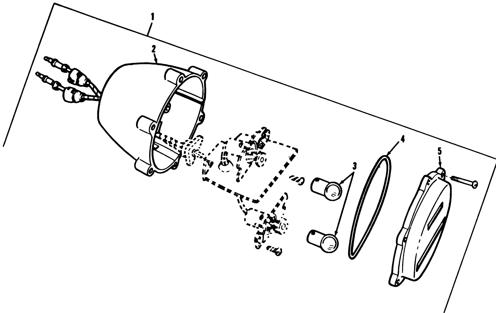
Figure 25. Stoplight—taillight assembly (right).
