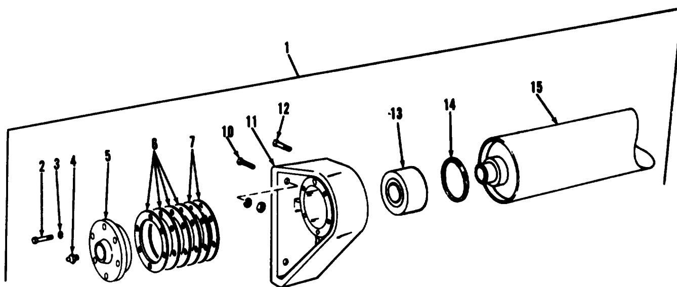
Figure 148. Loading roller.
