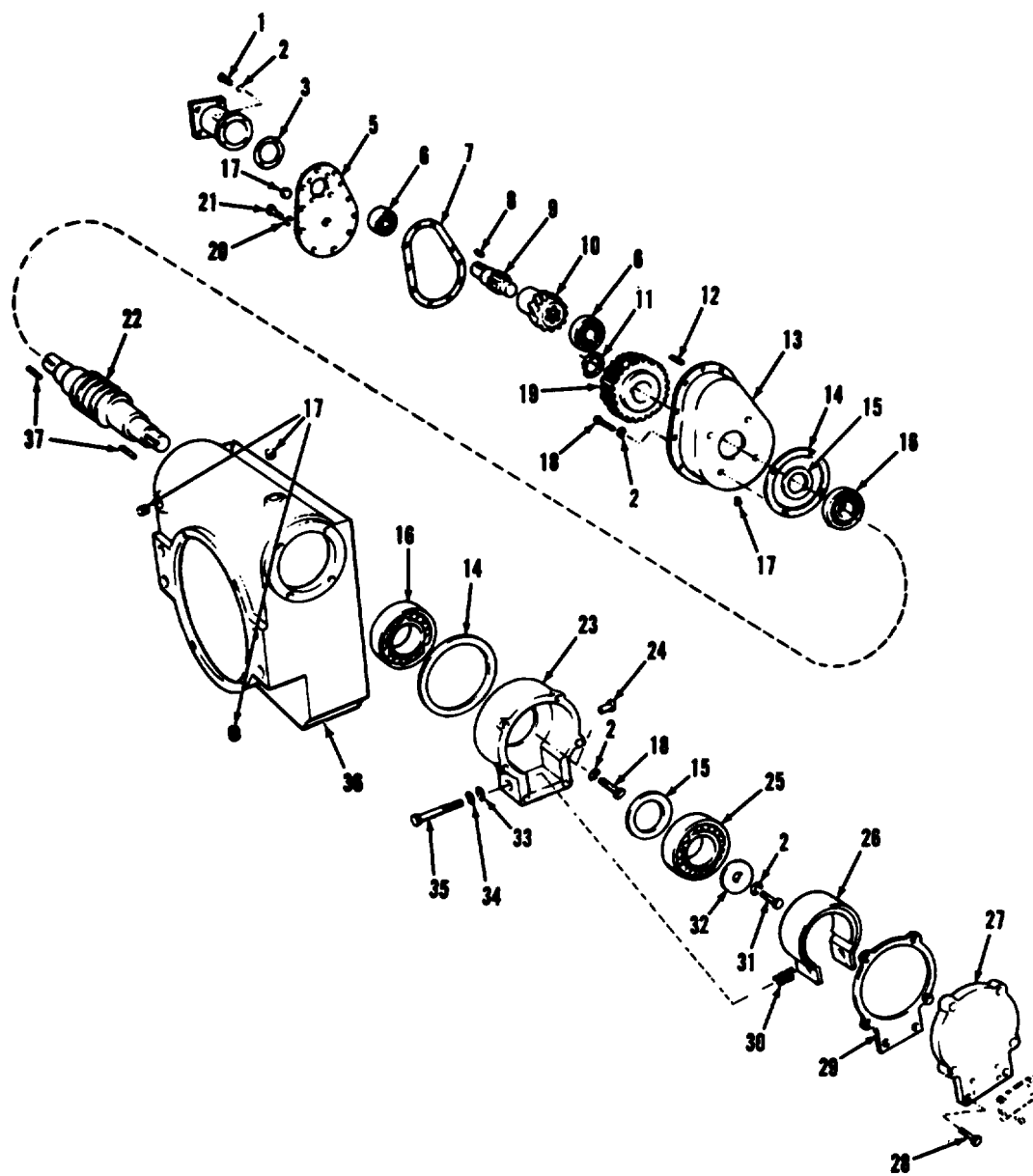
Figure 259. Hoist winch.
