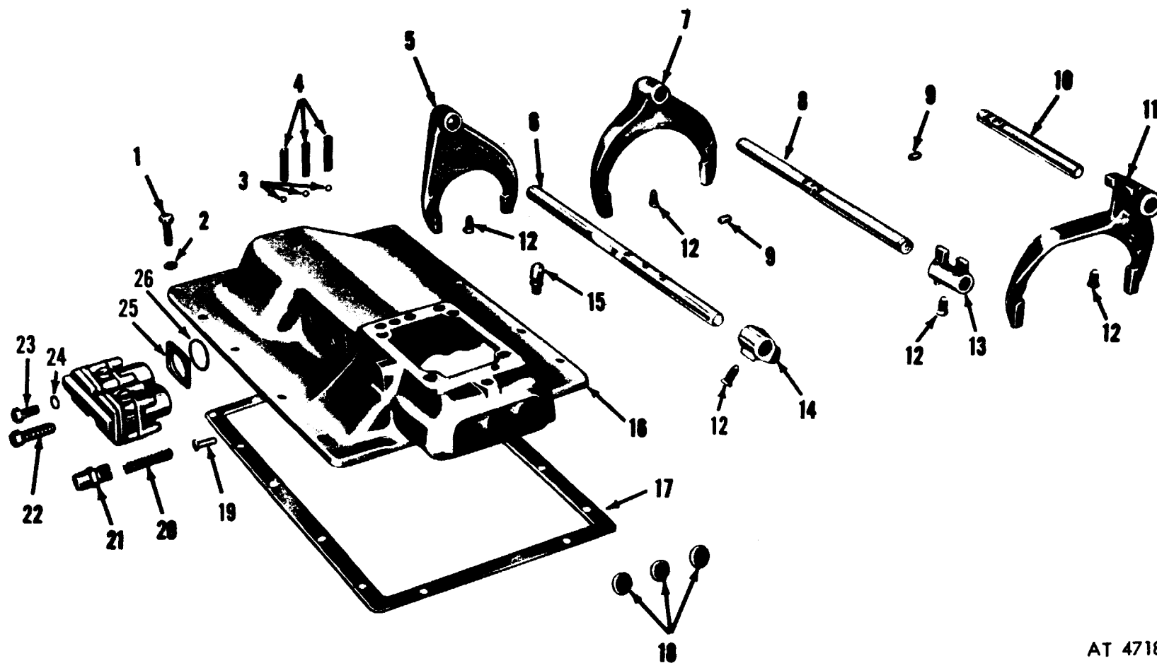
Figure 48. Transmission shifter housing and related parts.
