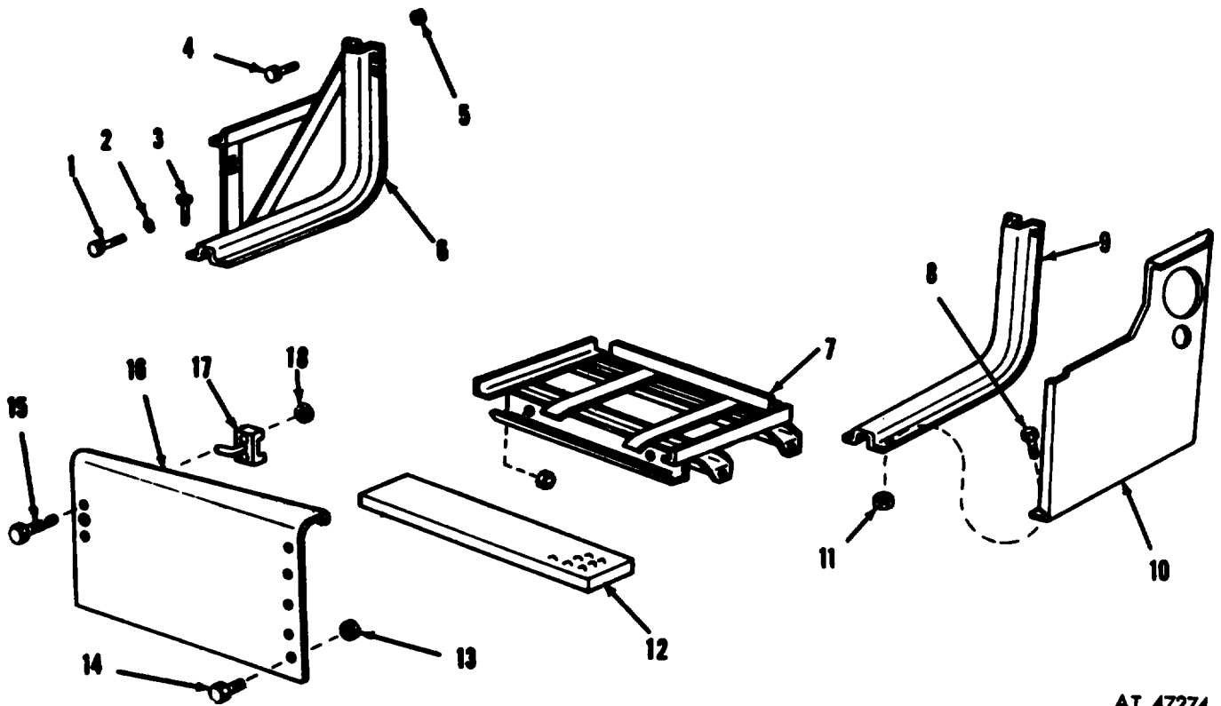
Figure 134. Right running board and related parts.
