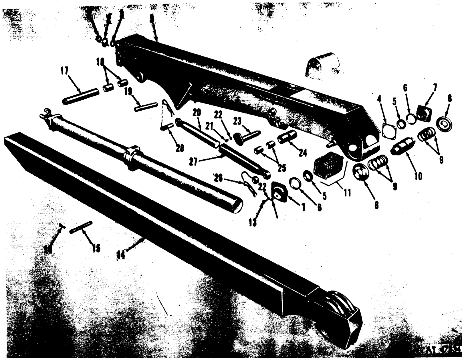
Figure 243. Boom and shipper.
