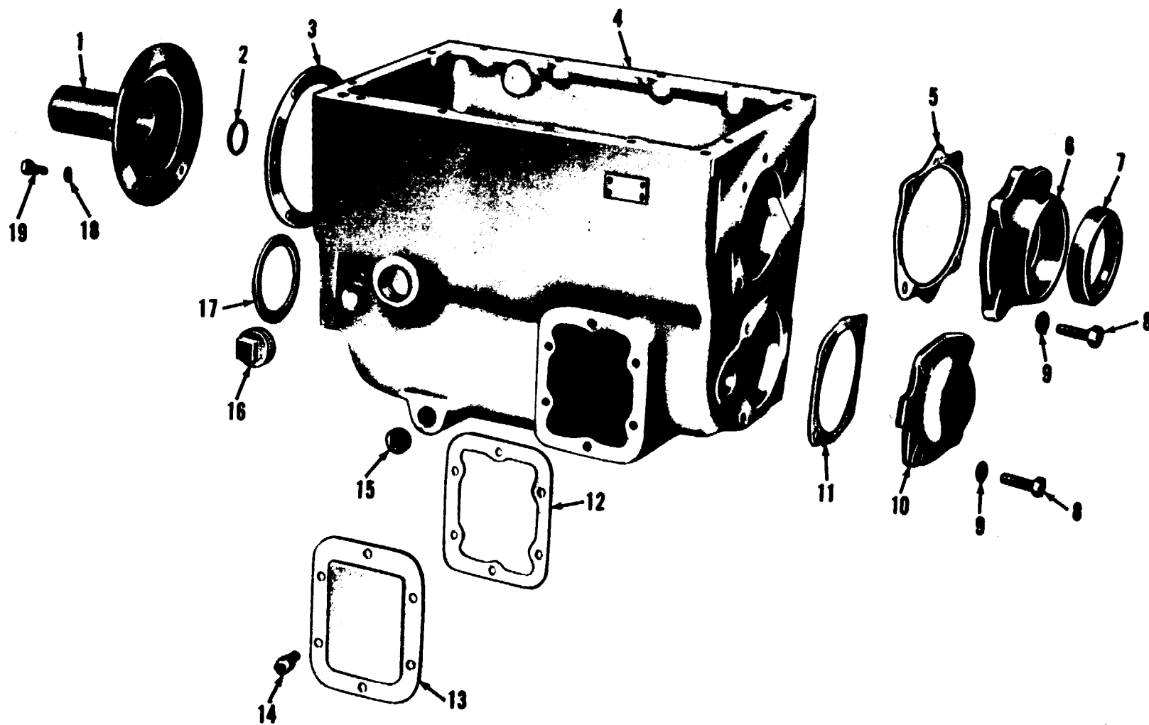
Figure 42. Transmission case and attaching parts.
