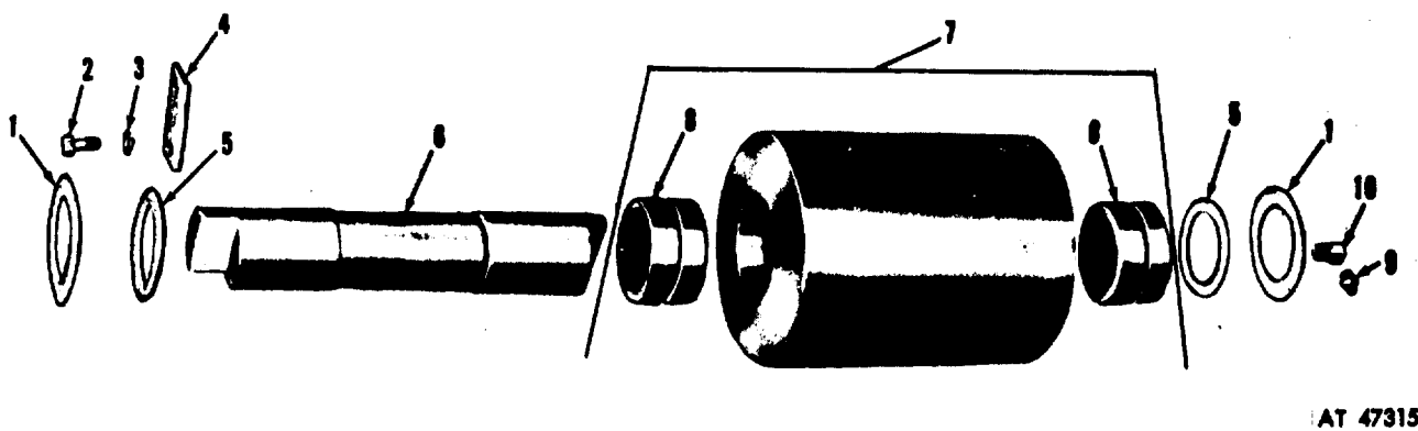
Figure 220. Rear winch upper and lower roller.
