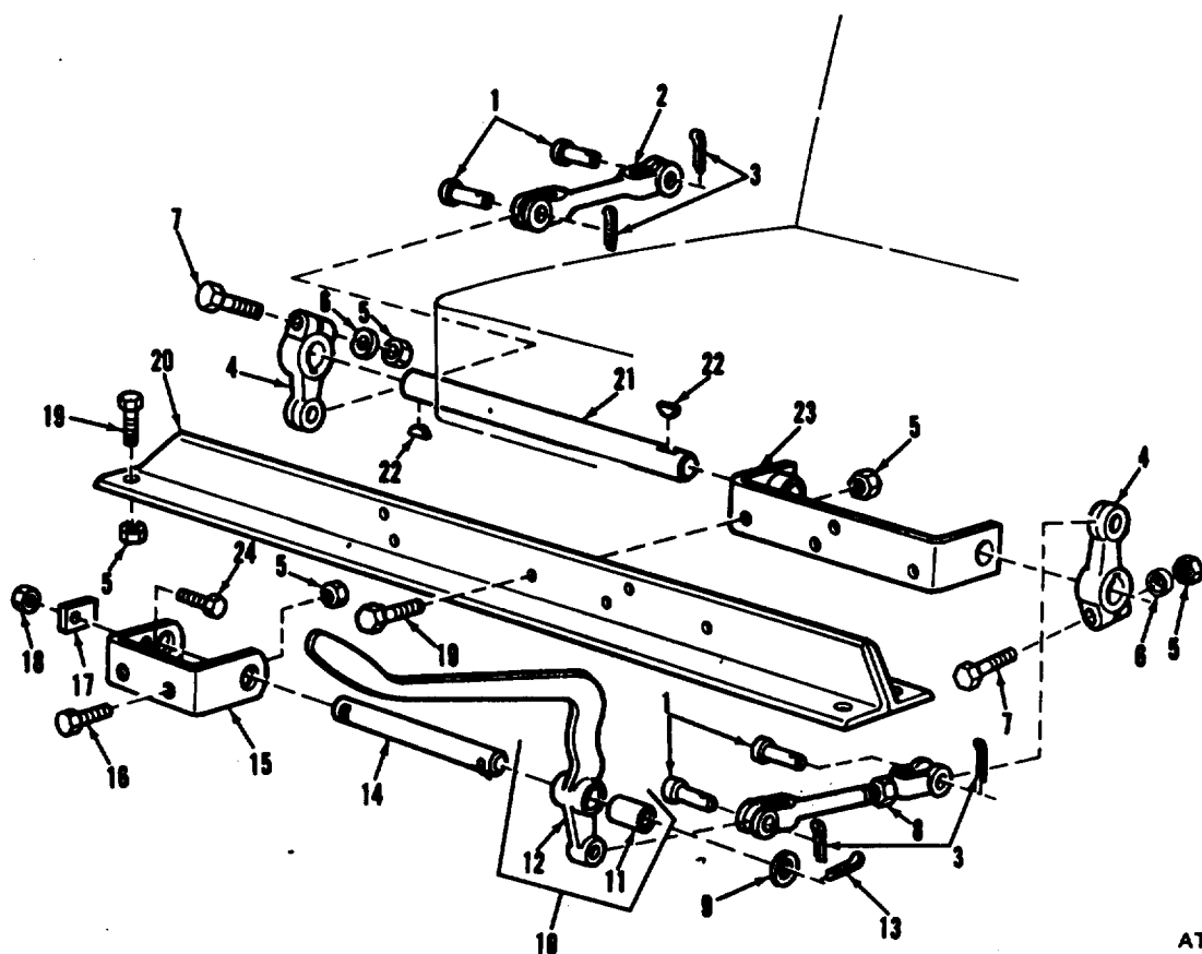
Figure 58. Transfer controls.
