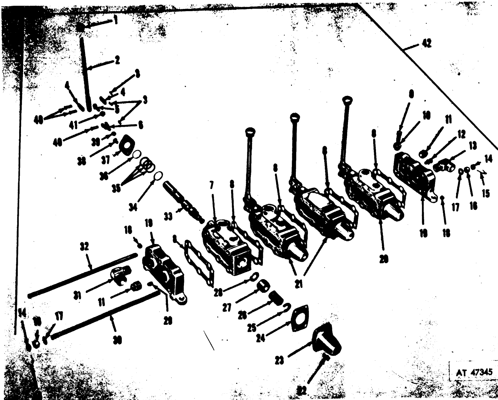
Figure 254. Control valve bank.
