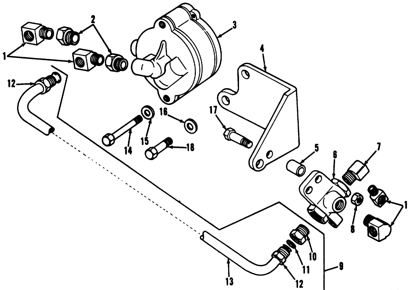
Figure 272. Power divider winch governor and related parts.
