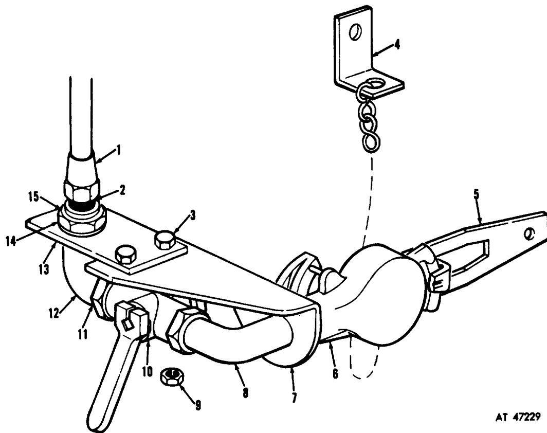
Figure 90. Trailer connections.
