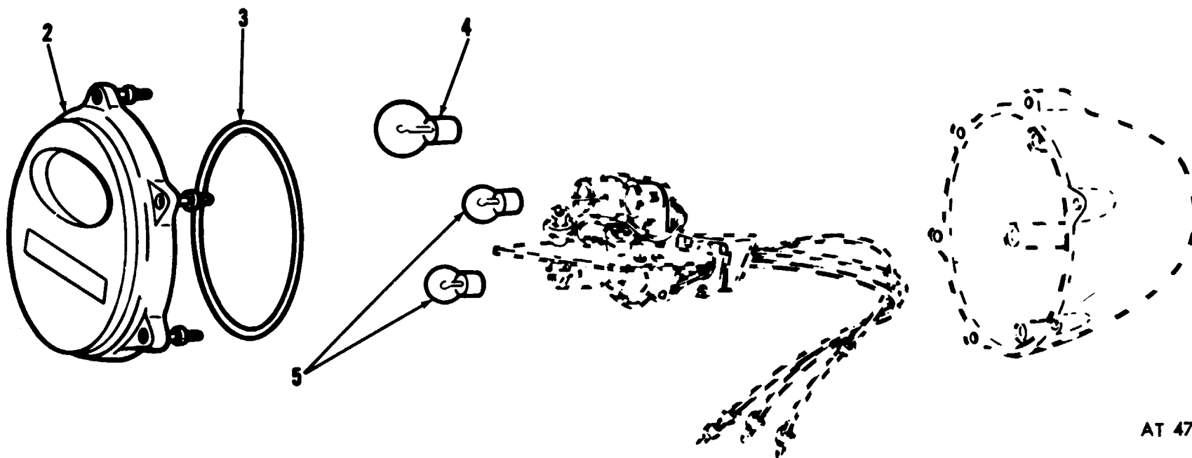
Figure 26. Stoplight—taillight assembly (left).
