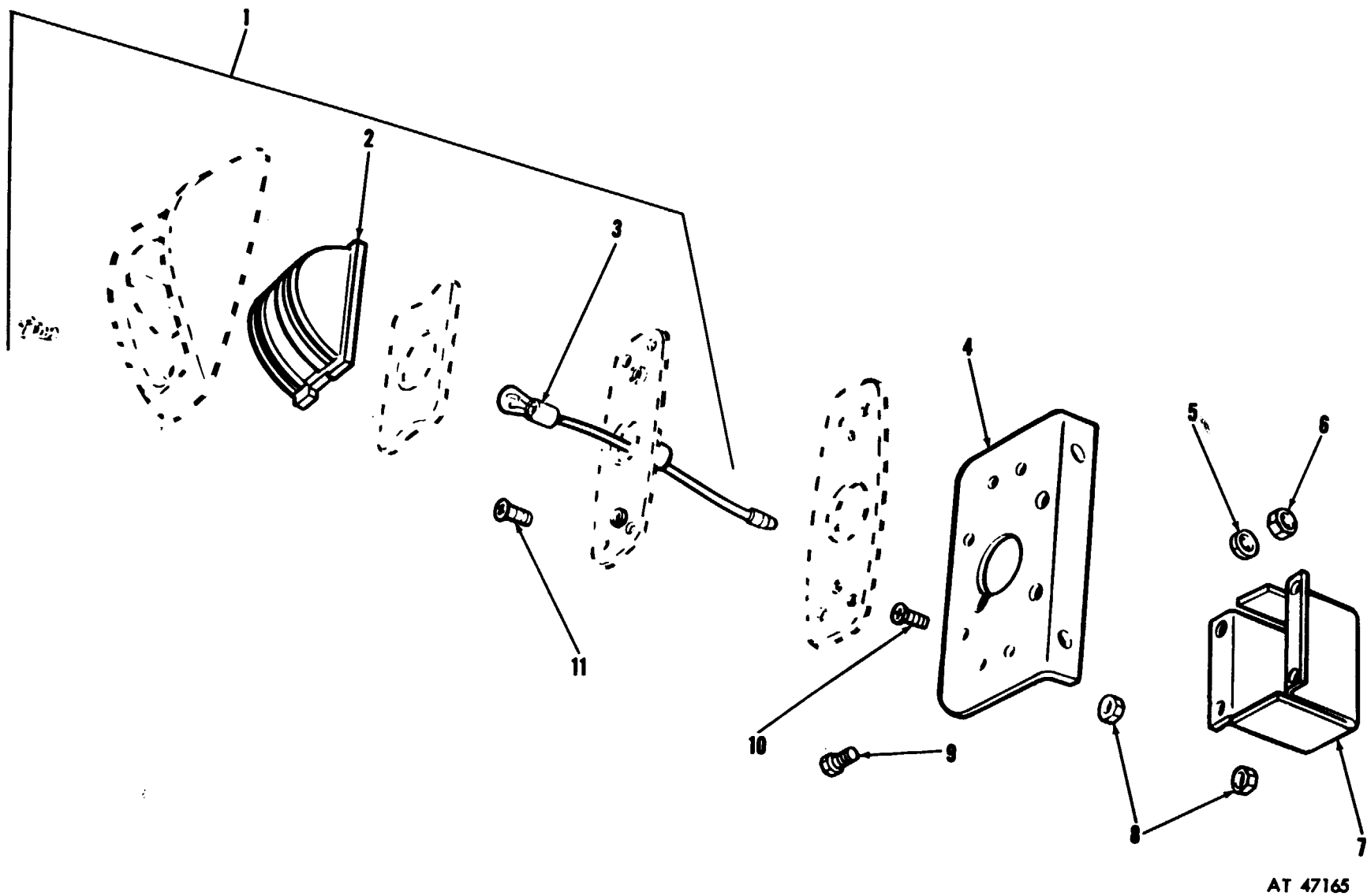
Figure 24. Marker light assembly (special lighting).
