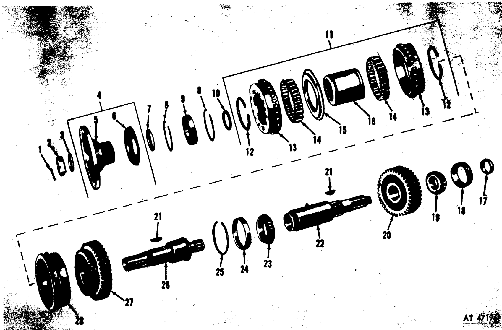
Figure 56. Transfer output shafts and related parts.
