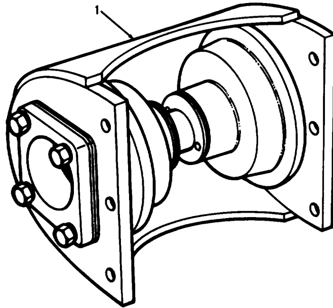
Figure 245. Upper roller shipper assembly.
