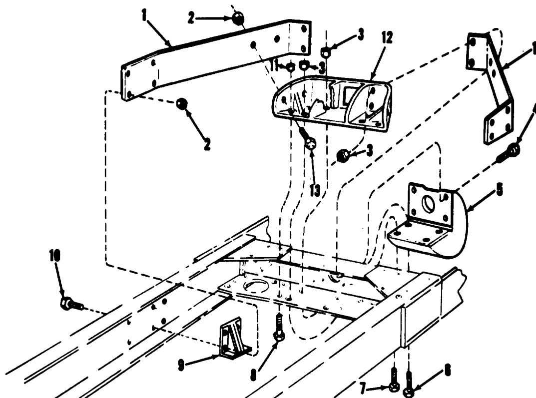
Figure 113. Pintle mounting installation.
