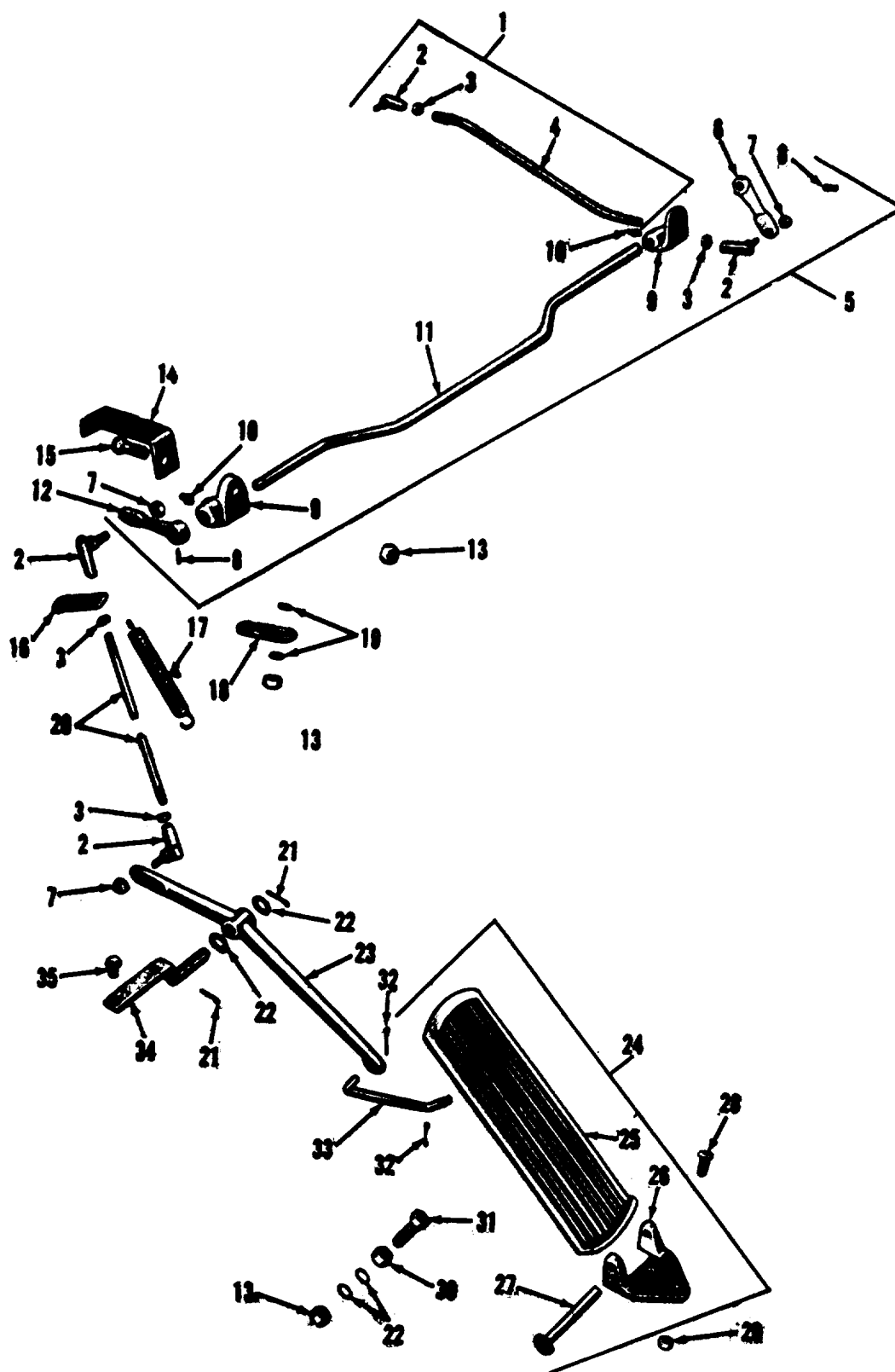
Figure 10. Throttle linkage.
