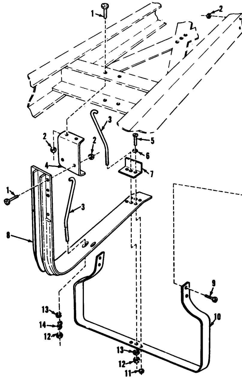
Figure 116. Tire carrier.
