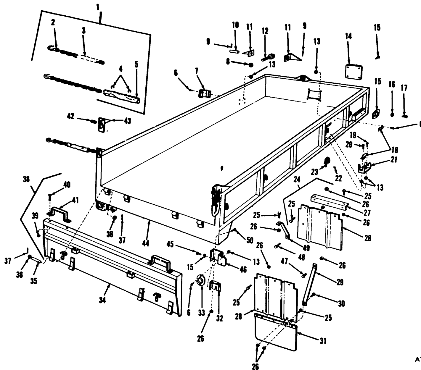
Figure 149. Cargo body.
